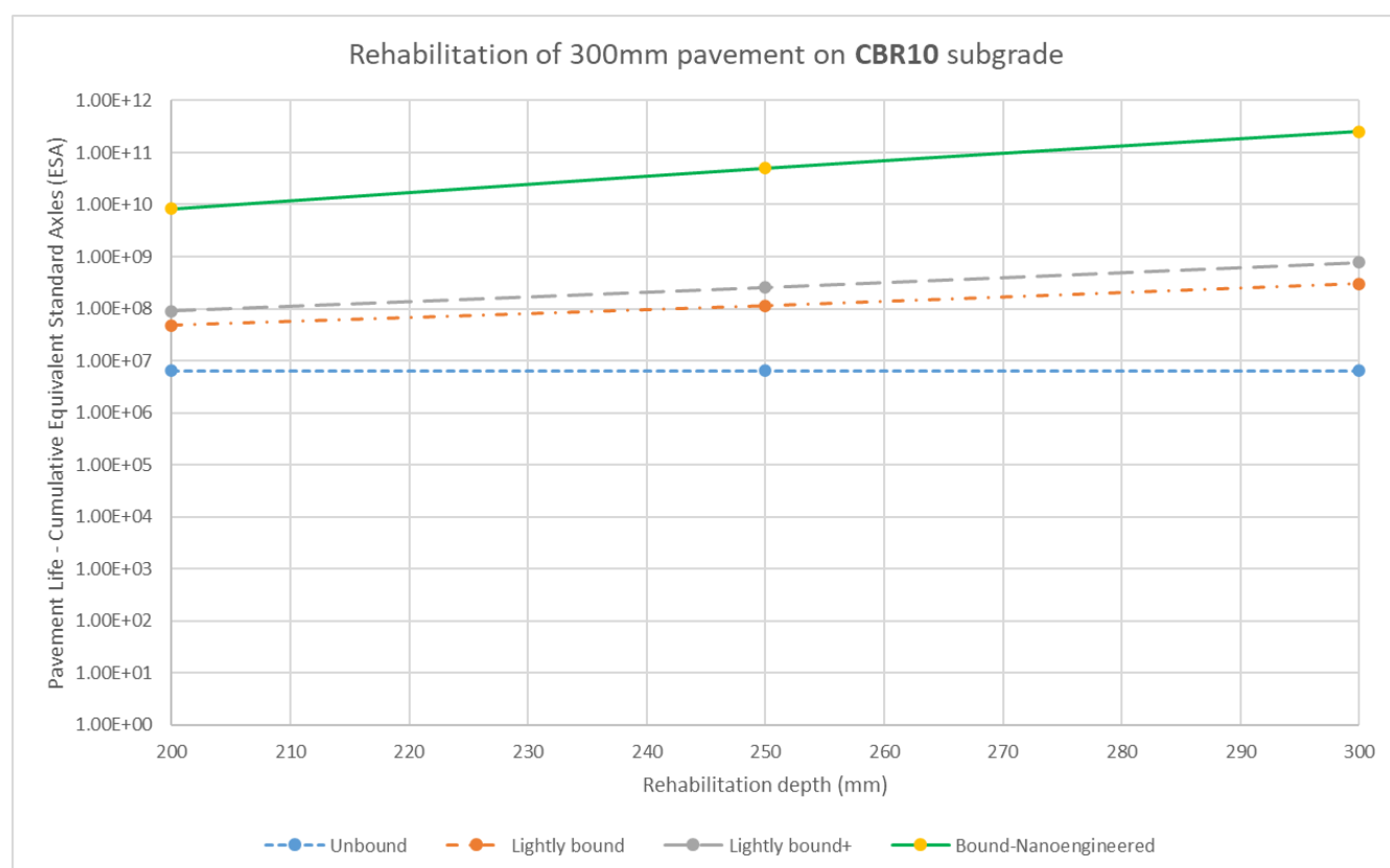
Figure 14: AustPADS outputs - Rehabilitation of 300mm pavement on CBR10 subgrade
