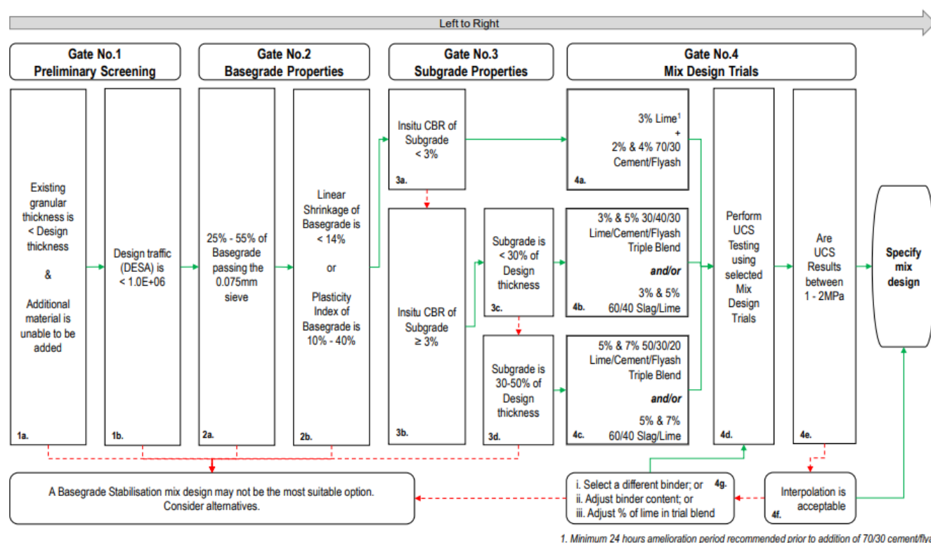
Figure 16 - Mix Design Procedure for Basegrade Stabilisation (from Young [15])
