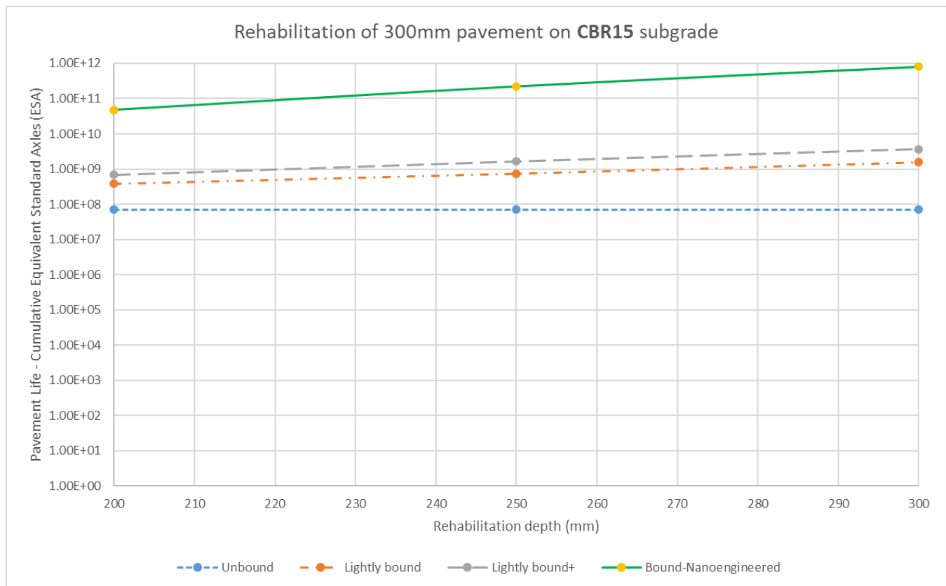
Figure 15: AustPADS outputs - Rehabilitation of 300mm pavement on CBR15 subgrade
