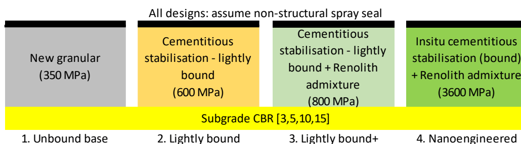
Figure 6: Pavement model 1 - New/rehabilitated base, no sub-base
