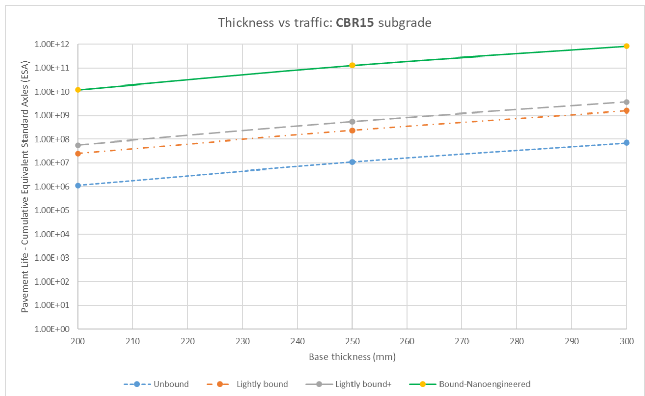
Figure 10: AustPADS outputs - New/rehabilitated base, no sub-base, CBR15 subgrade
