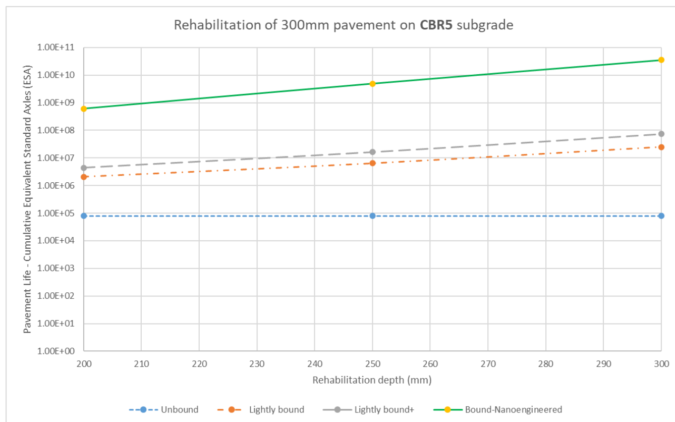
Figure 13: AustPADS outputs - Rehabilitation of 300mm pavement on CBR5 subgrade
