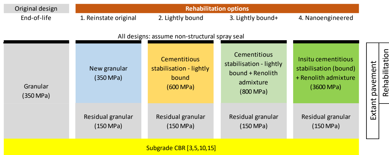
Figure 11: Pavement model 2: Rehabilitation of 300mm pavement
