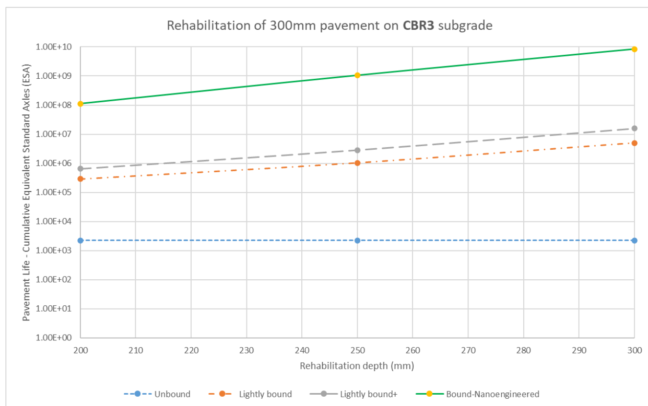
Figure 12: AustPADS outputs - Rehabilitation of 300mm pavement on CBR3 subgrade
